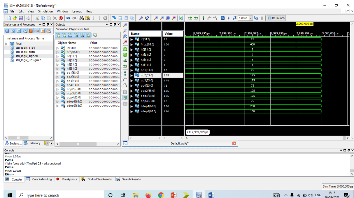
Fig7: proposed radix16 multiplier based FIR filter
