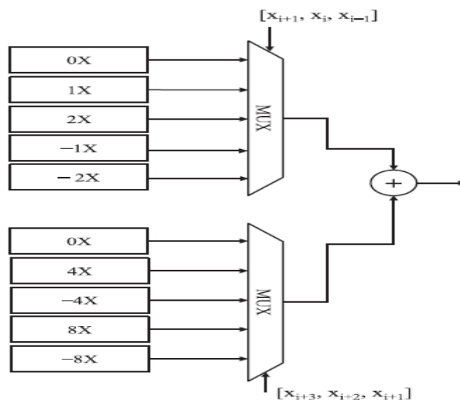
Fig5. Radix16 modified booth encoder
