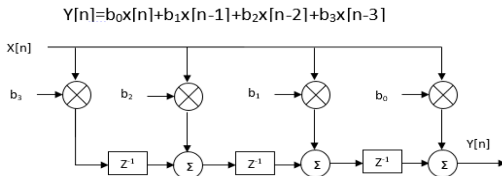
Fig1: DIGITAL FIR FILTER
